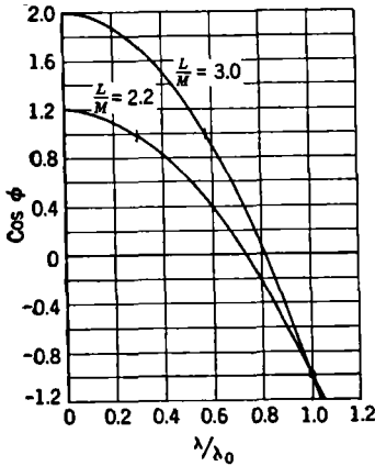
FIG. 4-6.— \text{Cos } \phi as a function of \lambda/\lambda_0 for a chain of shunt-resonant circuits with mutual coupling. Values of \text{cos } \phi > 1 correspond to \phi imaginary. \lambda_0 is 2\pi c\sqrt{LC} .
